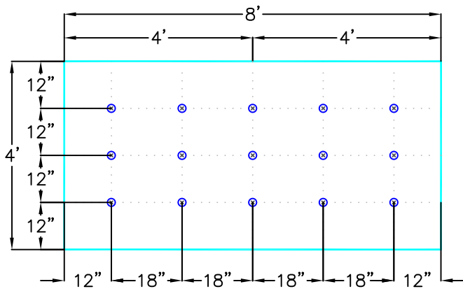
FM 1-90 (PERIMETER) ENHANCEMENT PATTERN
