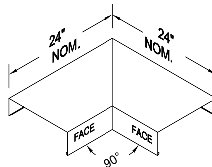
INSIDE MITER
